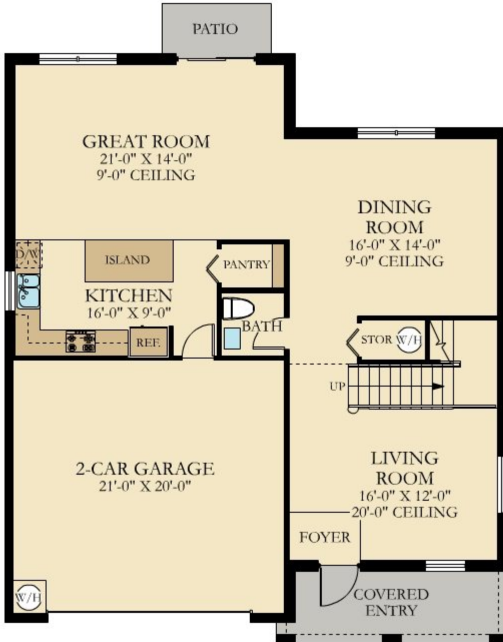
FIRST FLOOR
