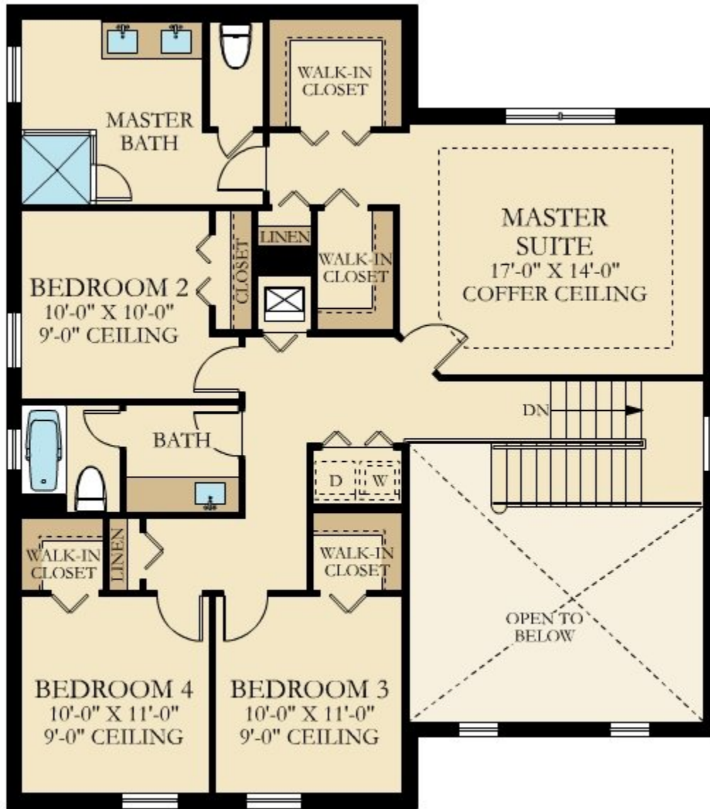
SECOND FLOOR
