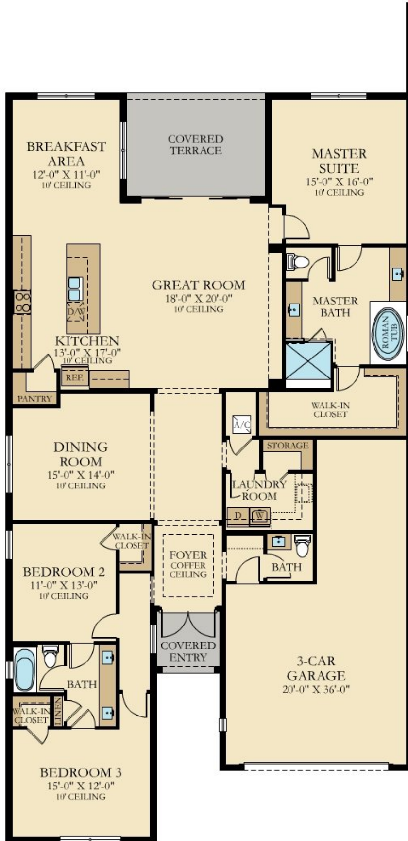
FIRST FLOOR
