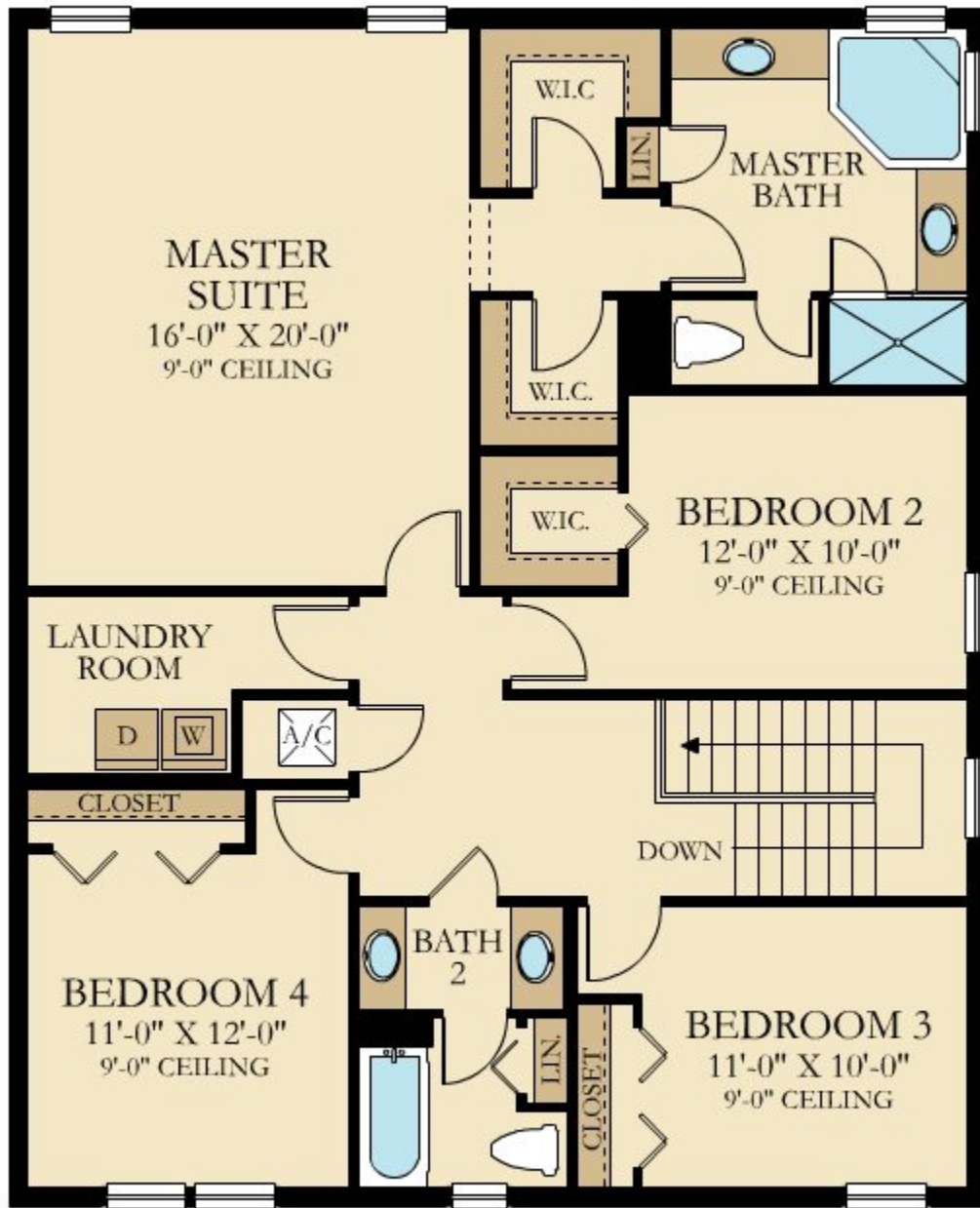
SECOND FLOOR
