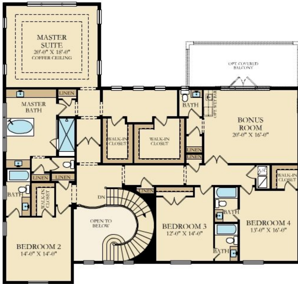
SECOND FLOOR
