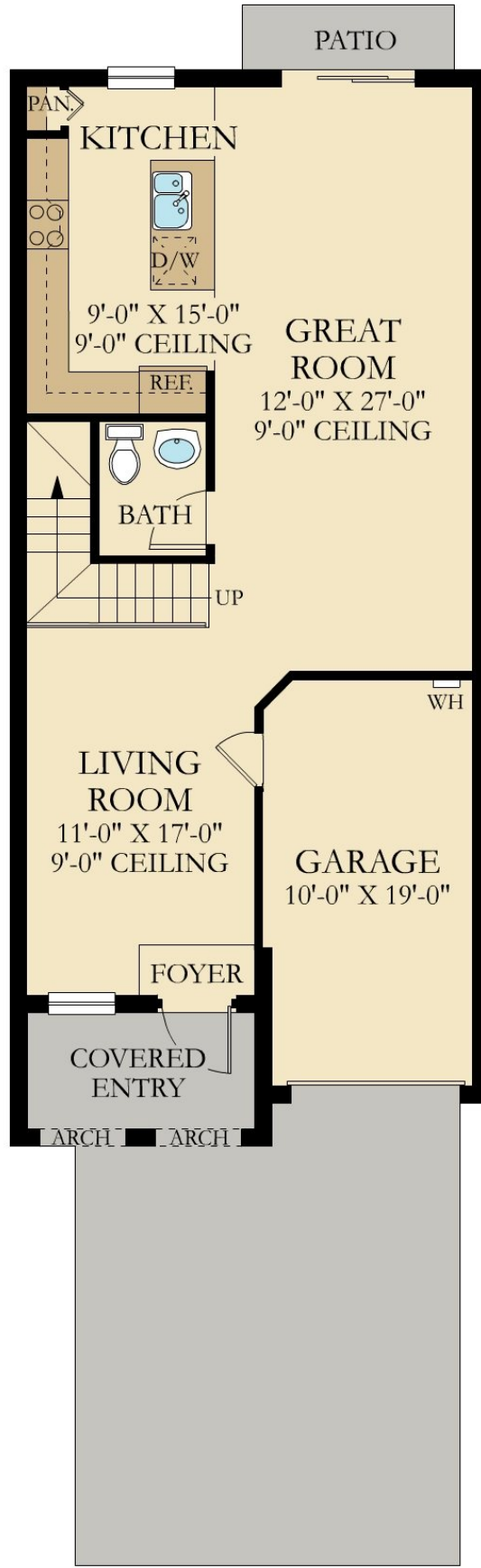
FIRST FLOOR
