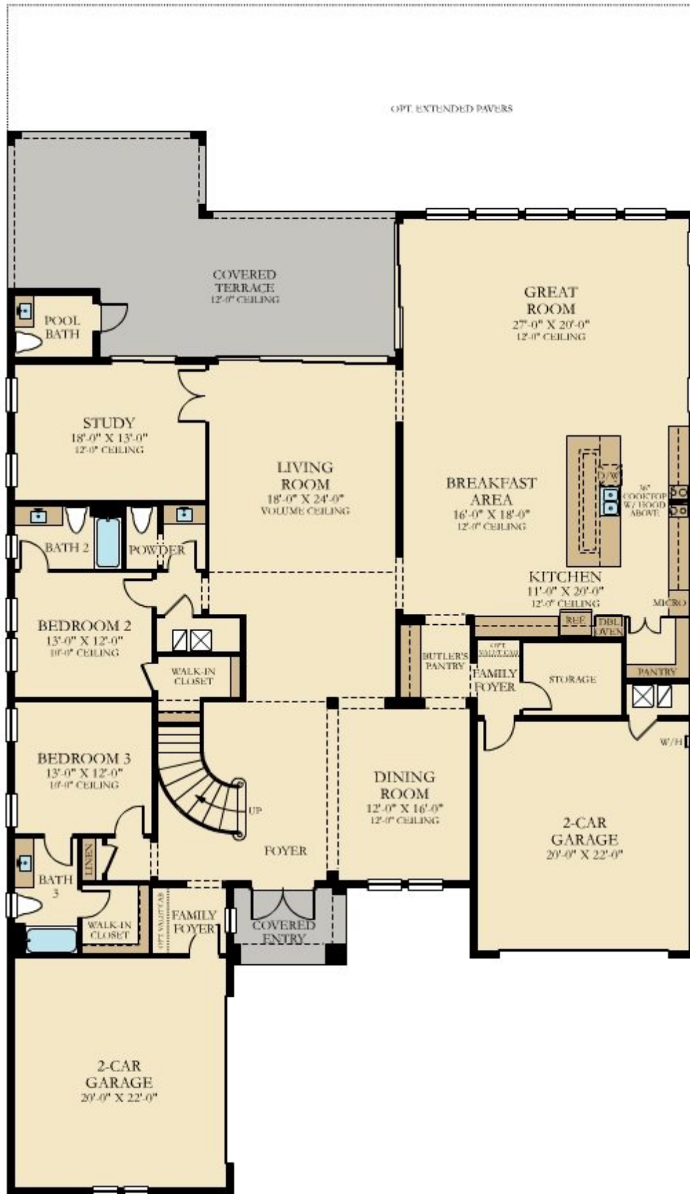
FIRST FLOOR
